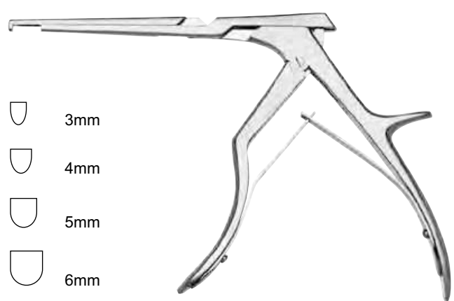
SPURLING-KERRISON Rongeur Forceps Down-cutting bite. Jaw opening 15mm.
